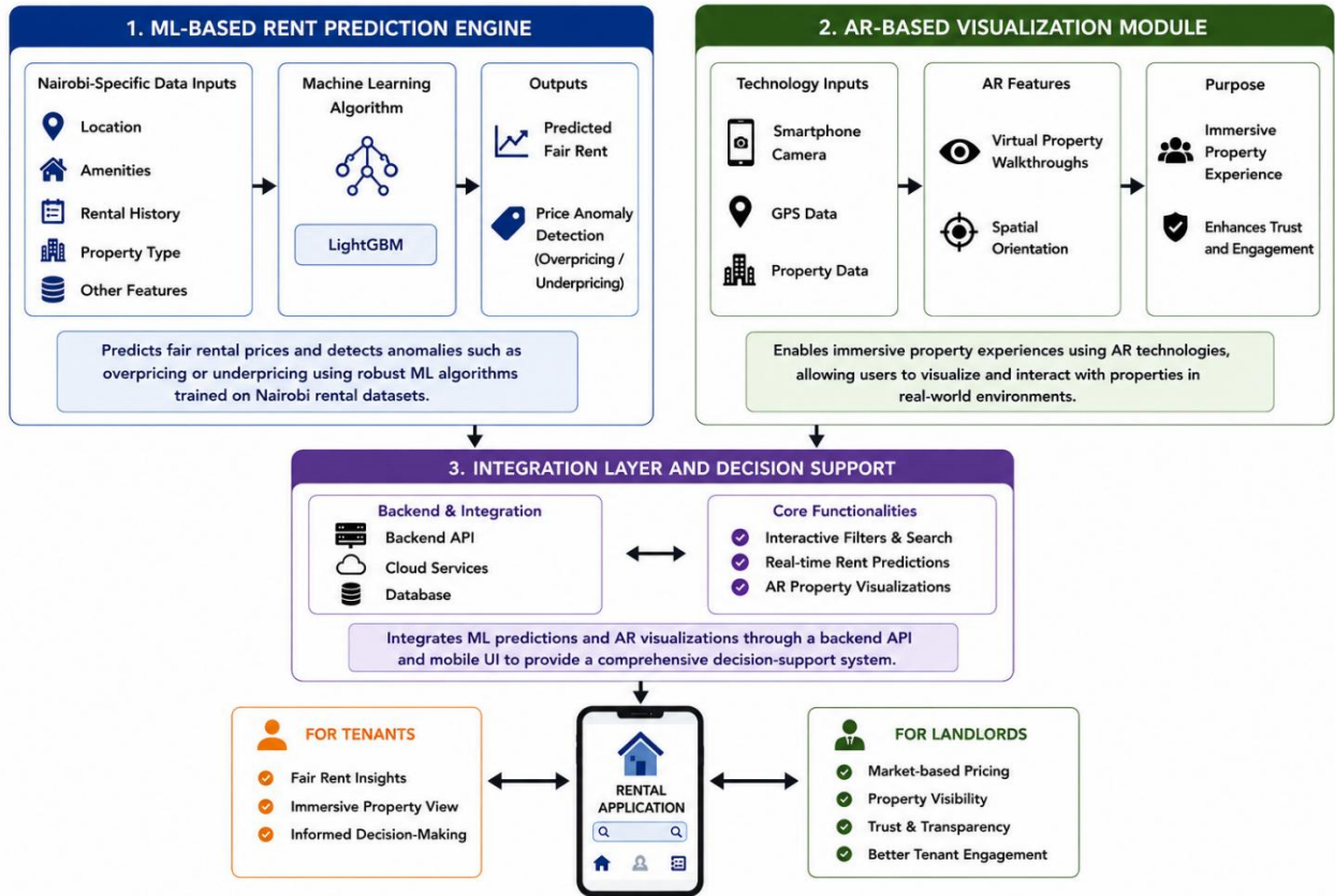
Figure 2. 6: Conceptual Framework for ML+ AR Rental Application
