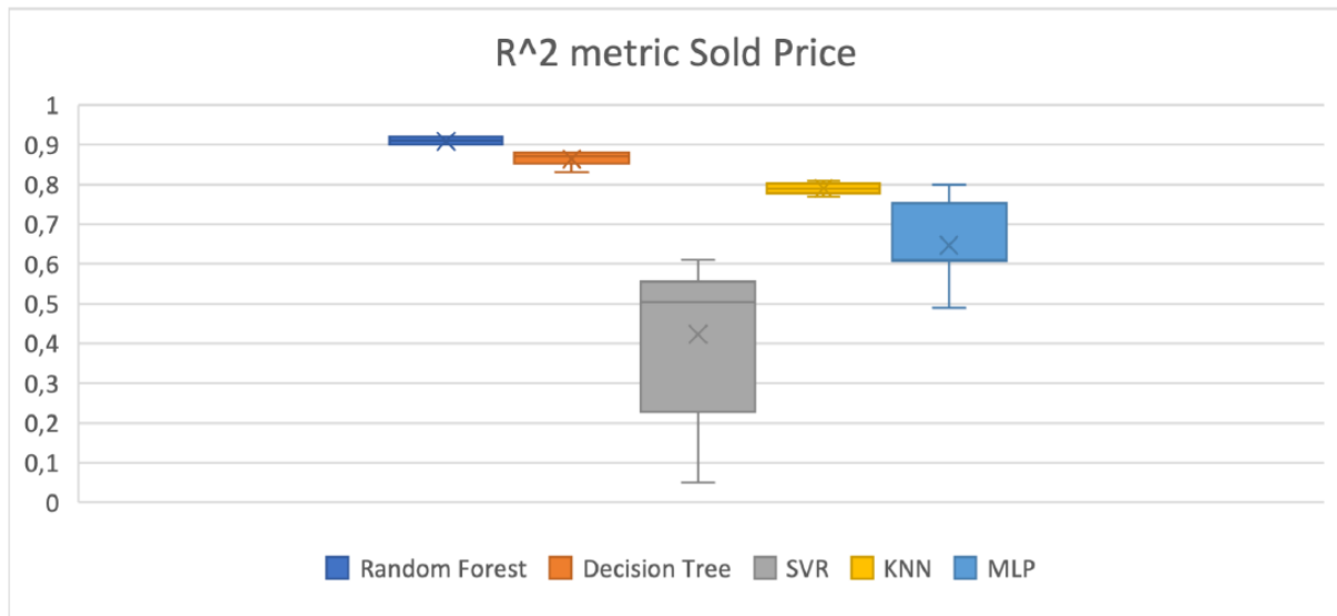
Figure 2. 3: Model performance comparison for housing price prediction (Eren, 2023)
