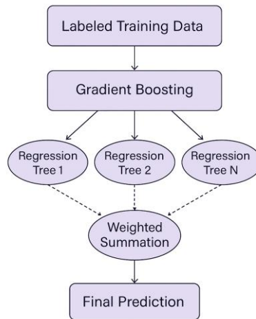
Figure 3. 1: Working process of LightGBM
